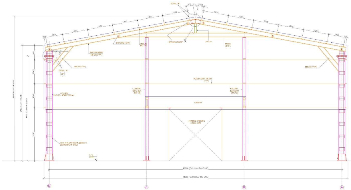
CROSS SECTION @ GRID LINE 1 & 6
