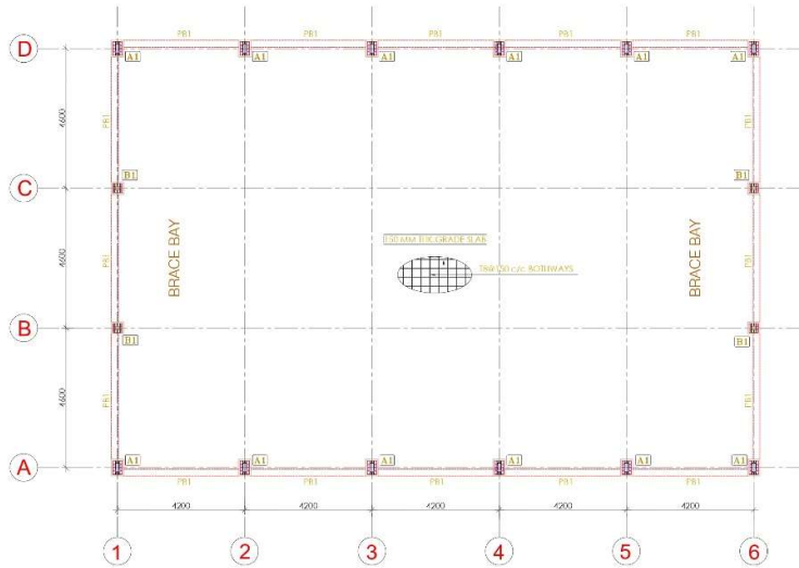
PLINTH BEAM LAYOUT PLAN
